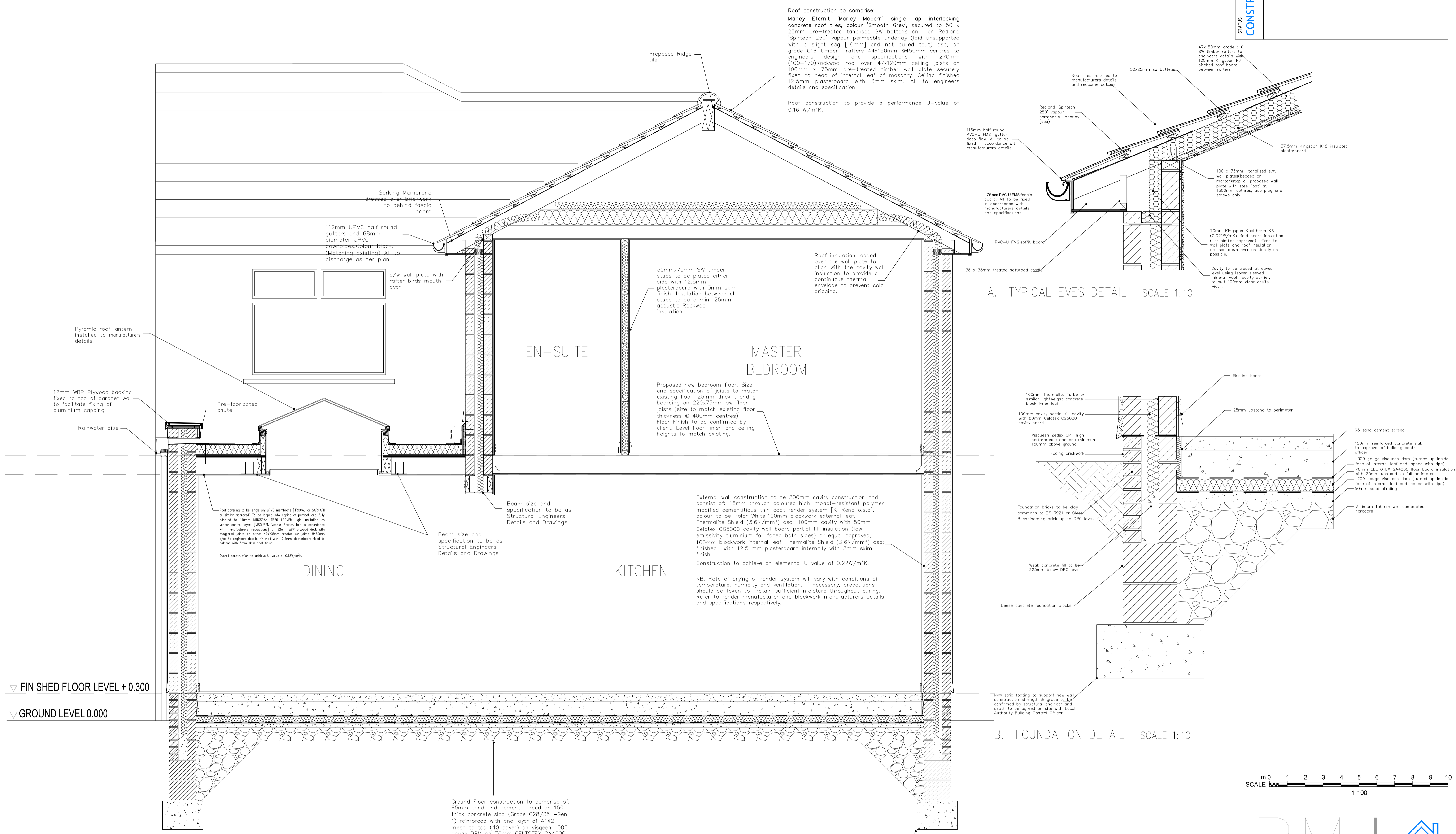
SECTION A-A | SCALE 1:20
